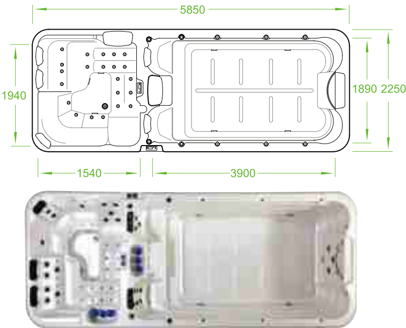
Model BG-6609 Overall Dimension 5850x2250x1400mm Interior Dimension Swim area : 3900x1890x1250mm Spa area : 1540x1940x820mm
