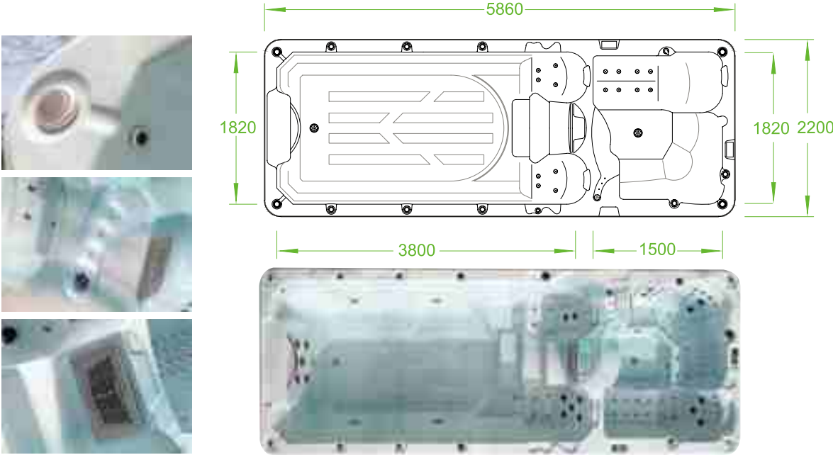
Model BG-6610 Overall Dimension 5860x2200x1300mm Interior Dimension Swim area : 3800x1820x1150mm Spa area : 1500x1820x790mm
