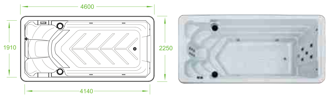
Model Overall Dimension Interior Dimension BG-6603 4600x 2250 x 1470mm 4140x1910x1330mm
