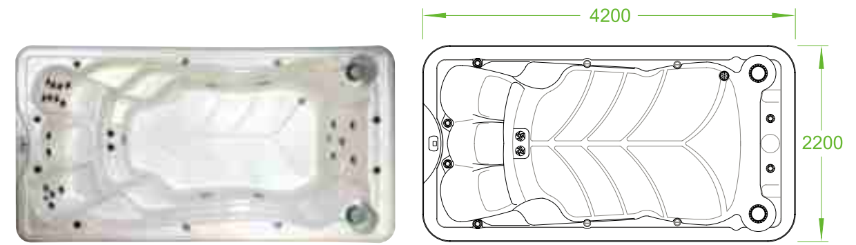
Model Overall Dimension Interior Dimension BG-6602 4200x2200x1450mm 3710x1840x1320mm
